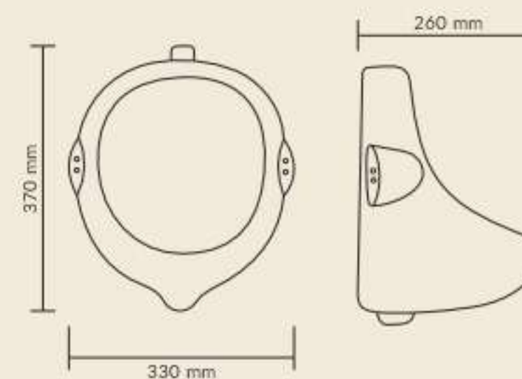
FLAT BACK Product : Urinal Dimensions : 330 X 260 X 370 mm
