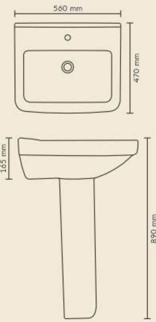
SYONA SET Product : Wash Basin With Pedestal (Capto) Dimensions : 560 X 470 X 890 mm (22" X 19" X 35")
