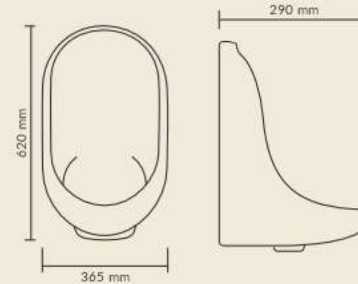
LARGE Product : Urinal Dimensions : 365 X 290 X 620 mm
