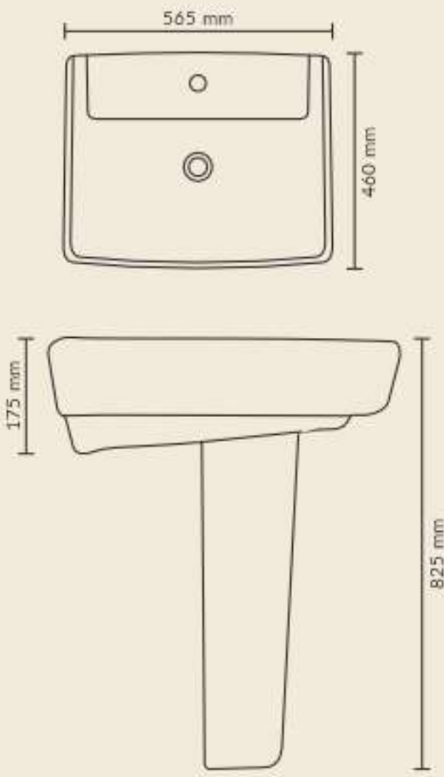
SONATA SET Product : Wash Basin With Pedestal (Capto) Dimensions : 565 X 460 X 825 mm (22" X 18" X 32")
