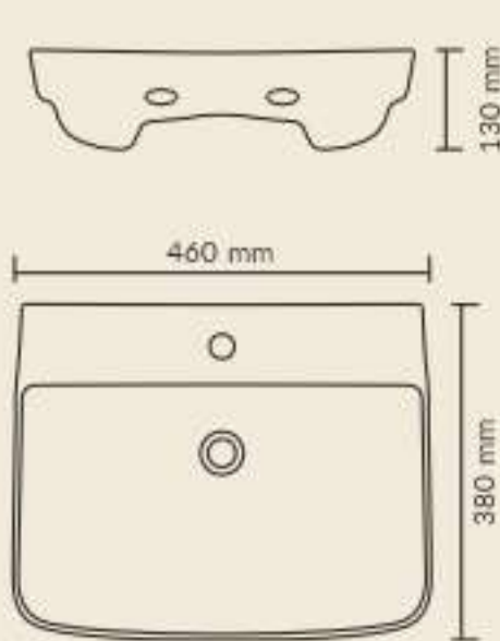
LICHI Product : Wash Basin Dimensions : 460 X 380 X 130 mm (18" X 15" X 5")
