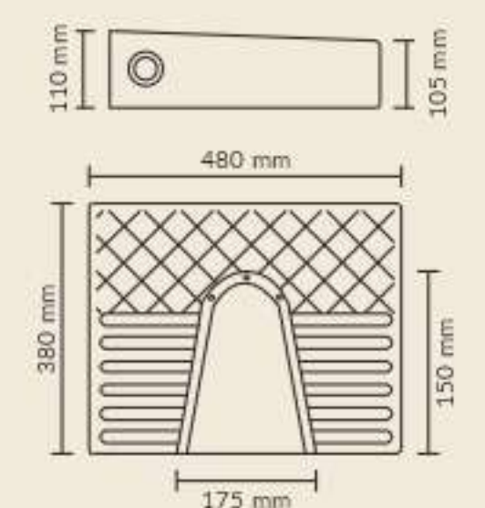
SQUATING Product : Urinal Dimensions : 480 X 380 X 110 mm
