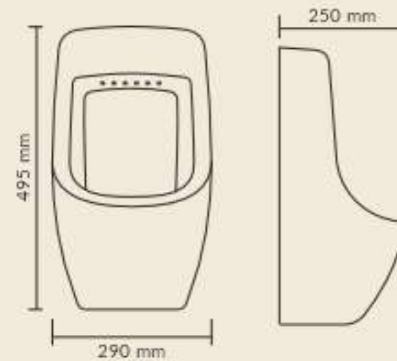
KODI Product : Urinal Dimensions : 290 X 250 X 495 mm
