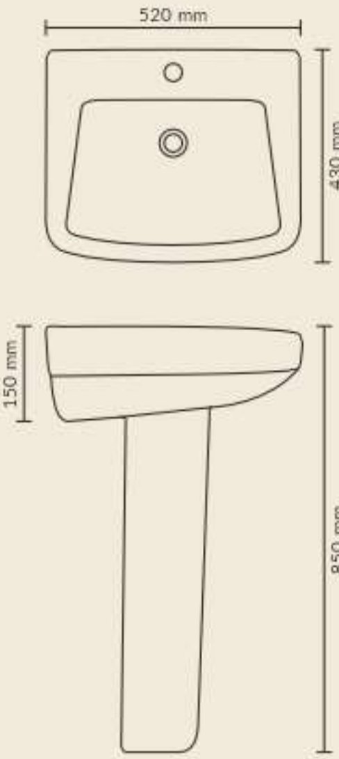
LORAL SET Product : Wash Basin With Pedestal (Capto) Dimensions : 520 X 430 X 850 mm (20" X 17" X 33")
