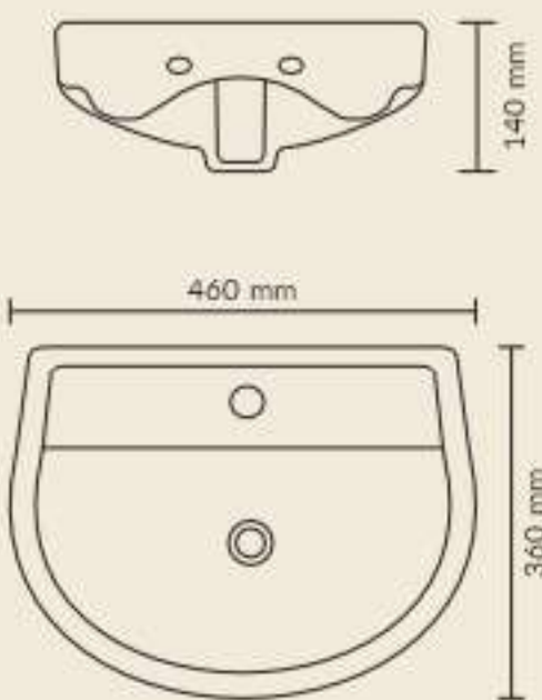
JEX Product : Wash Basin Dimensions : 460 X 360 X 140 mm (18" X 14" X 6")
