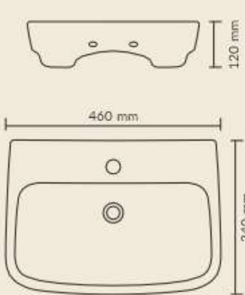
POLO Product : Wash Basin Dimensions : 460 X 340 X 120 mm (18" X 13" X 5")
