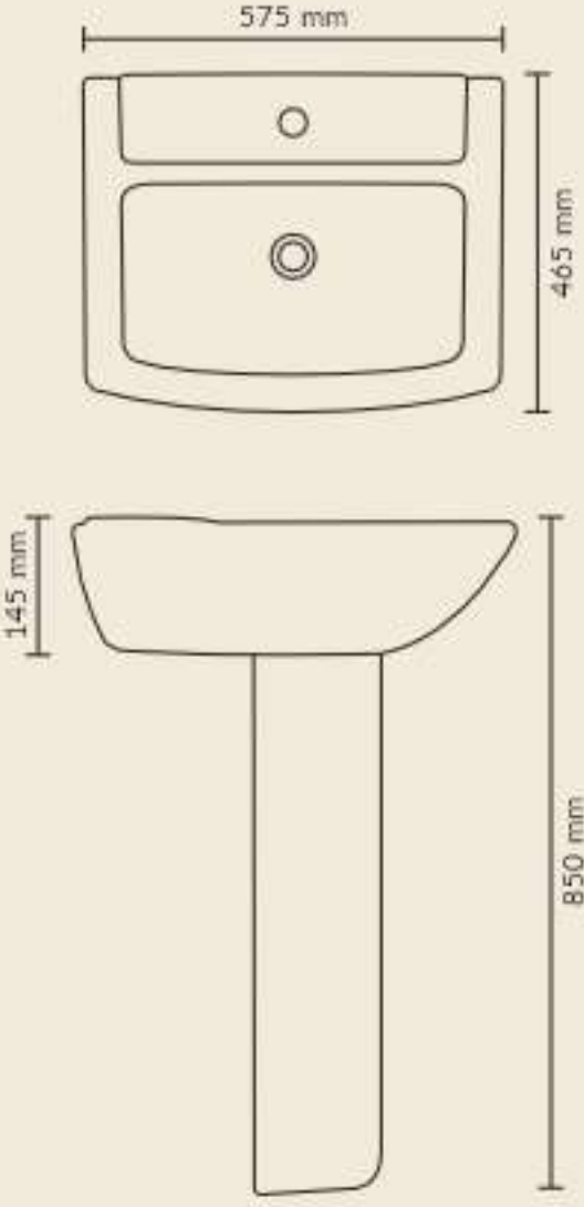
WIPRO SET Product : Wash Basin With Pedestal (Capto) Dimensions : 575 X 465 X 850 mm (23" X 18" X 33")
