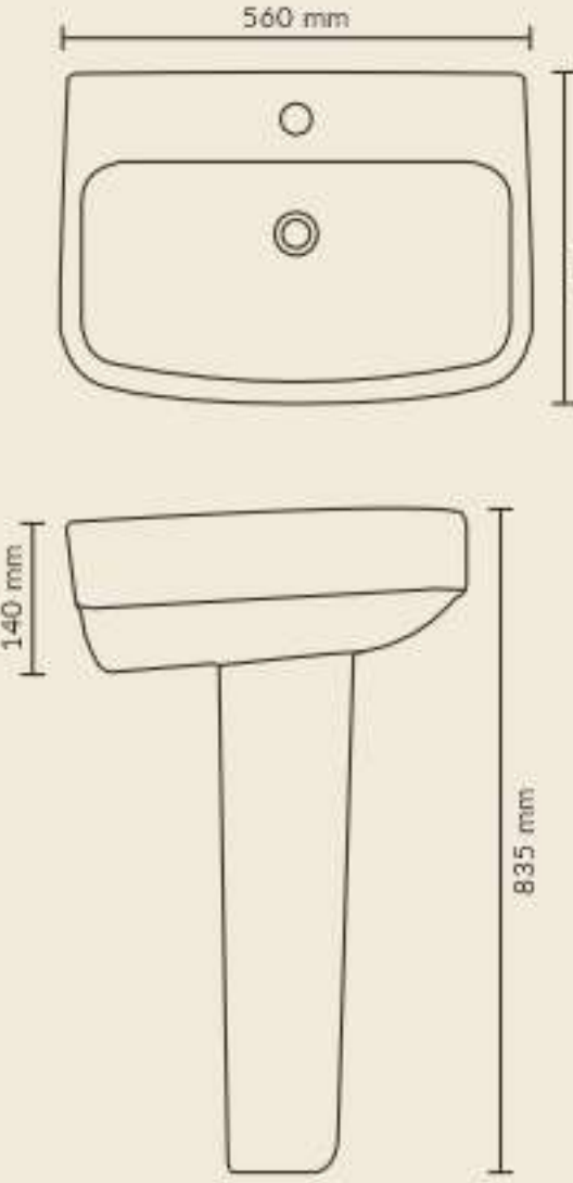
ORCHID SET Product : Wash Basin With Pedestal (Capto) Dimensions : 560 X 415 X 835 mm (22" X 16" X 33")
