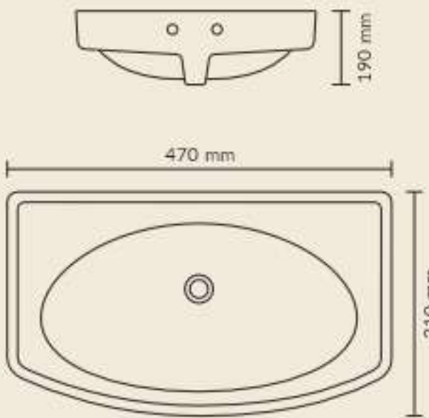
STEFEN Product : Wash Basin Dimensions : 470 X 310 X 190 mm (18" X 12" X 7")
