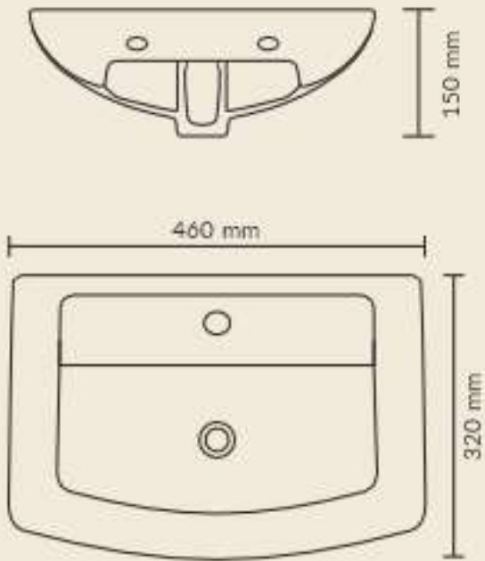
JET Product : Wash Basin Dimensions : 460 X 320 X 150 mm (18" X 13" X 6")
