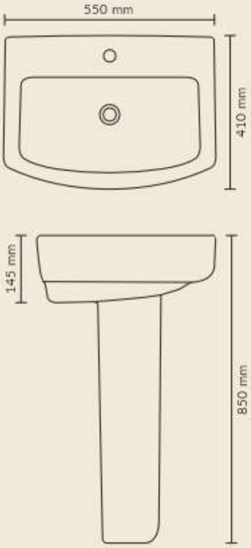
IRIS SET Product : Wash Basin With Pedestal (Capto) Dimensions : 550 X 410 X 850 mm (22" X 16" X 33")
