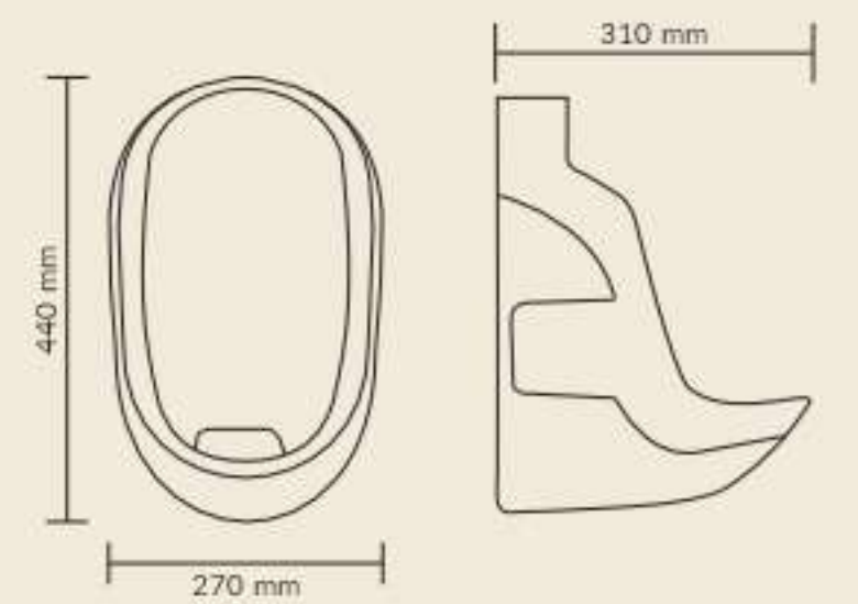
NANO LARGE Product : Urinal Dimensions : 270 X 310 X 440 mm
