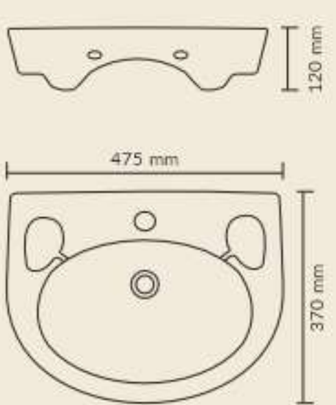
SUPER Product : Wash Basin Dimensions : 475 X 370 X 120 mm (19" X 15" X 5")
