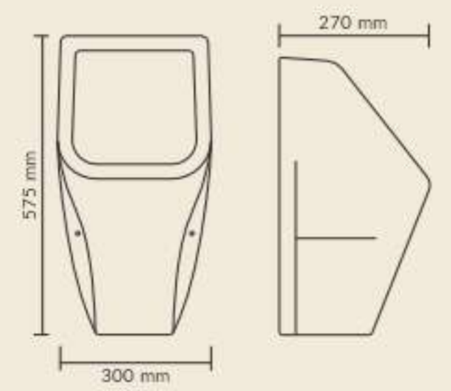
KIYAN Product : Urinal Dimensions : 300 X 270 X 575 mm
